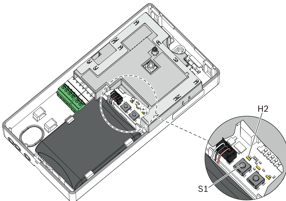
Figure 7.3: Radio gateway FWI-270
