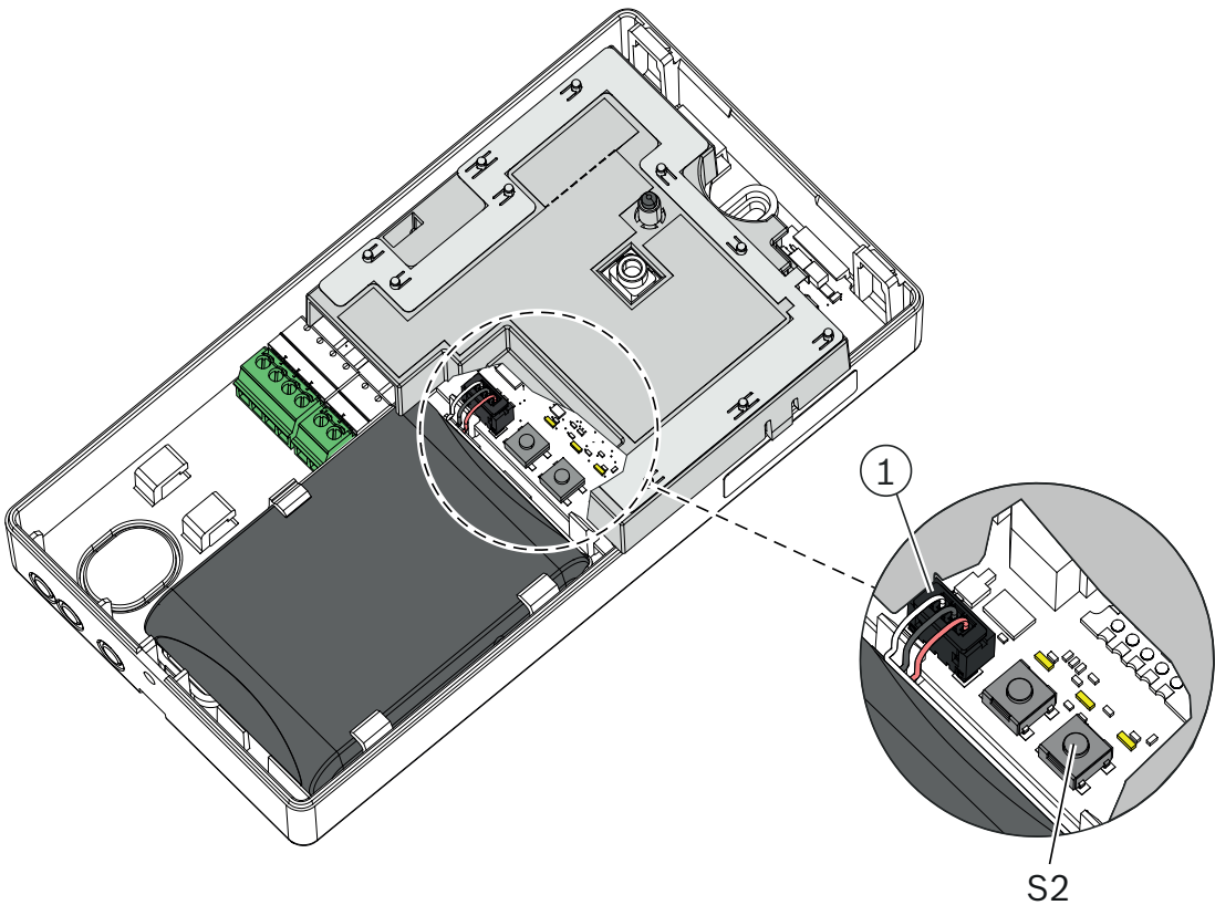
Figure 7.1: Radio gateway FWI-270
