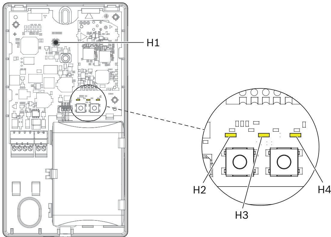
Figure 3.4: Radio gateway FWI-270
