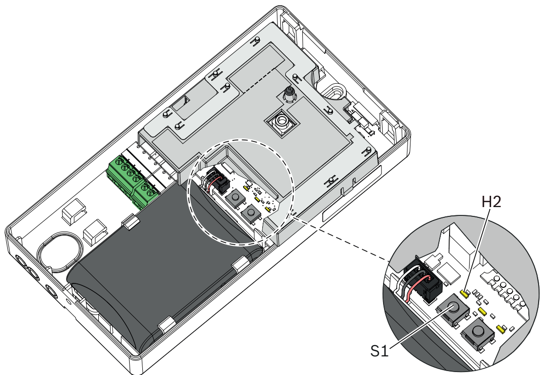
Figure 7.2: Radio gateway FWI-270
